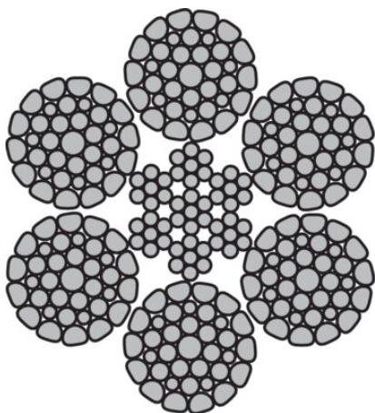
Winch rope
