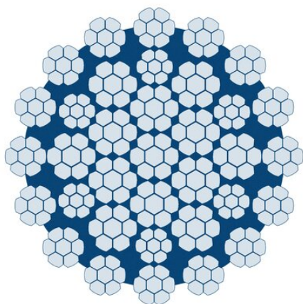
Tower crane
